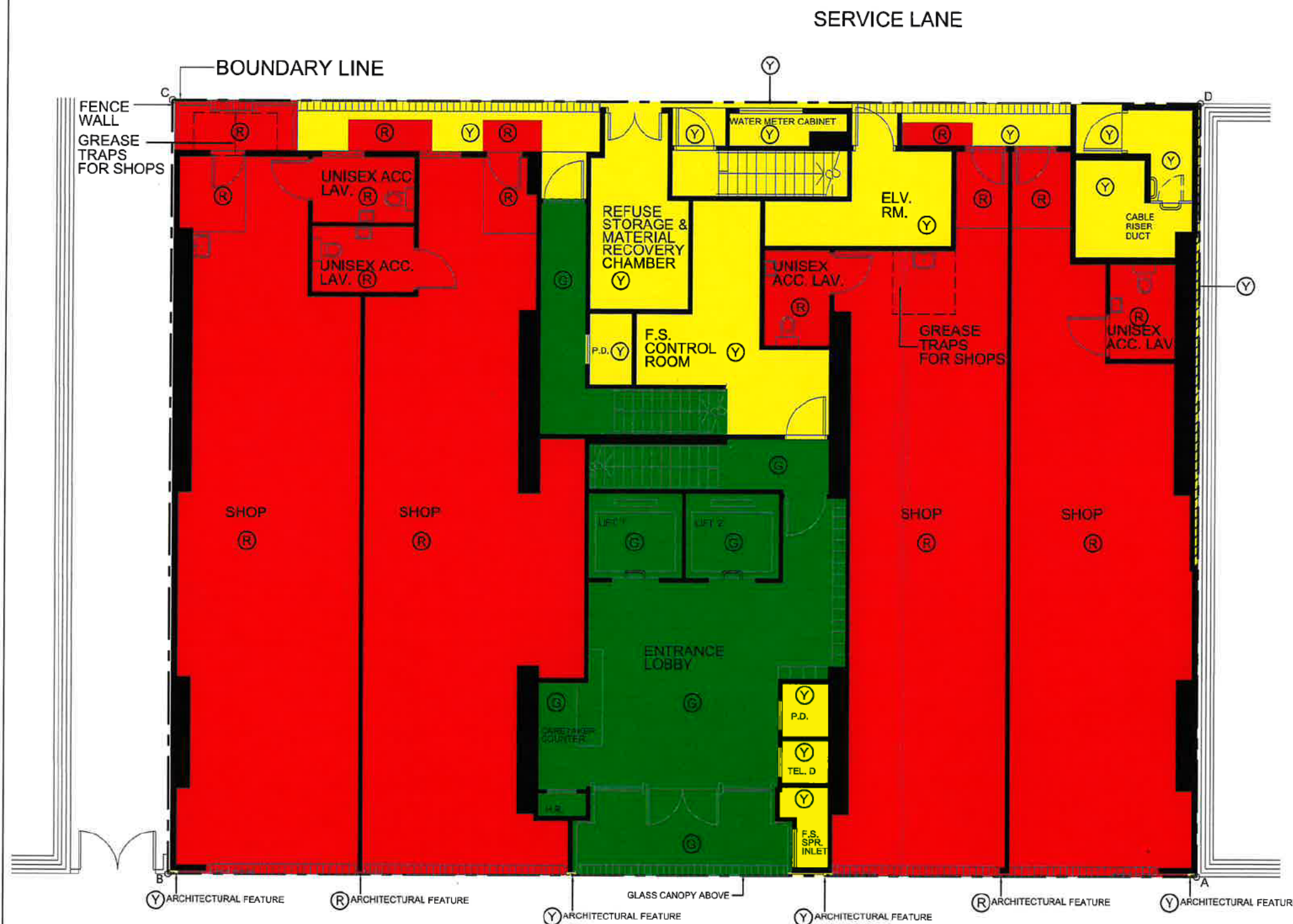
MAIN STREET, AP LEI CHAU GROUND FLOOR PLAN (PLAN NO. DMC - 01)
